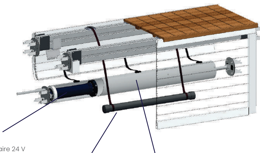
Kit contrepoids
